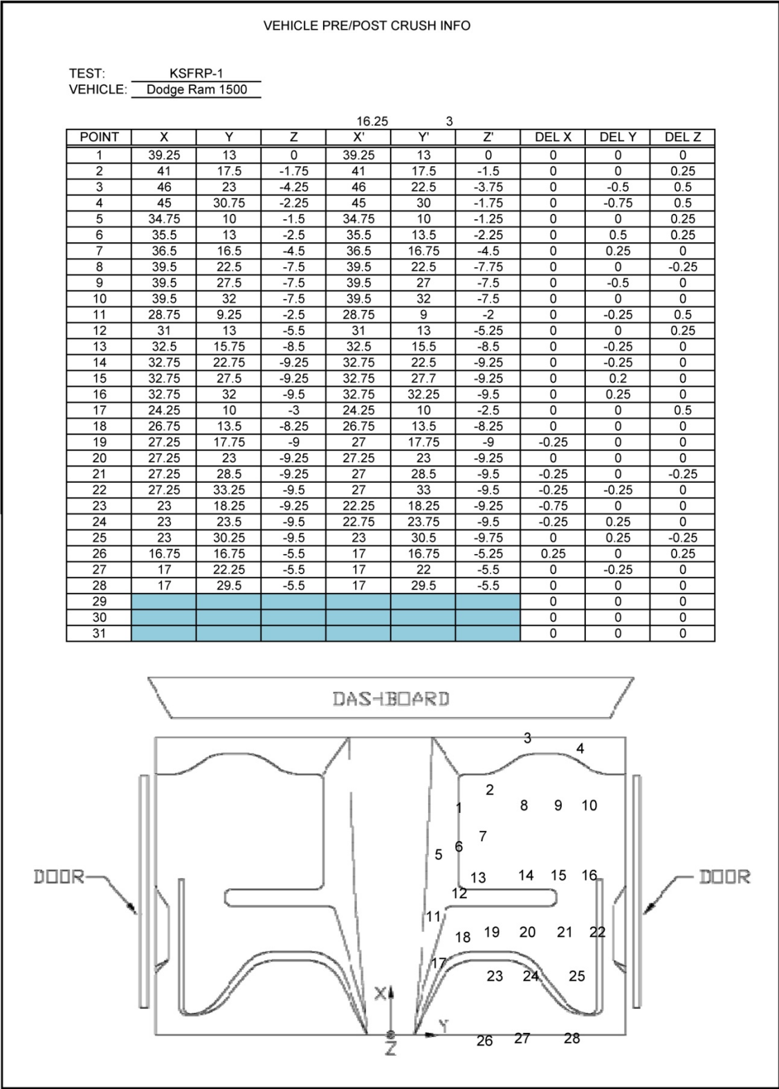
Figure C-2. Floor Pan Deformation Data – Set 2, Test No. KSFRP-1
